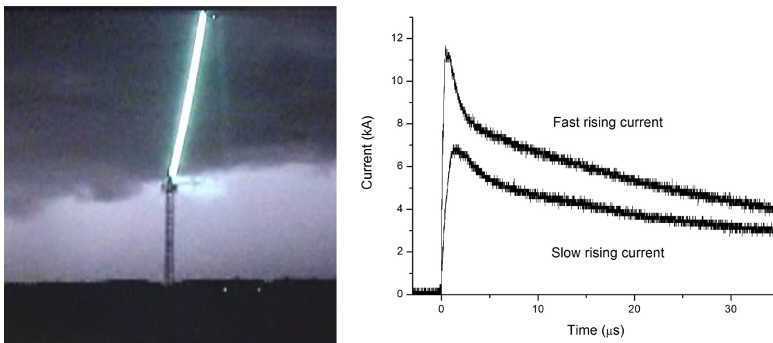
Figure I.2 – Photograph of rocket-triggered lightning and two current waveforms recorded at the tower top
