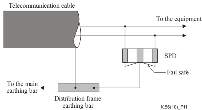
Figure 11 – Installation of SPD in the distribution frame
