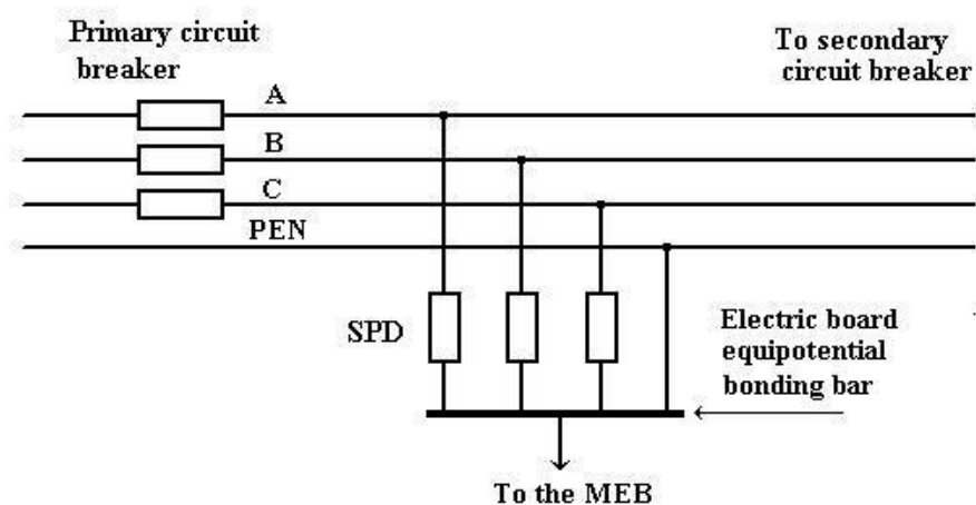
Figure 8 – Scheme for SPD installation on TN-C power systems
