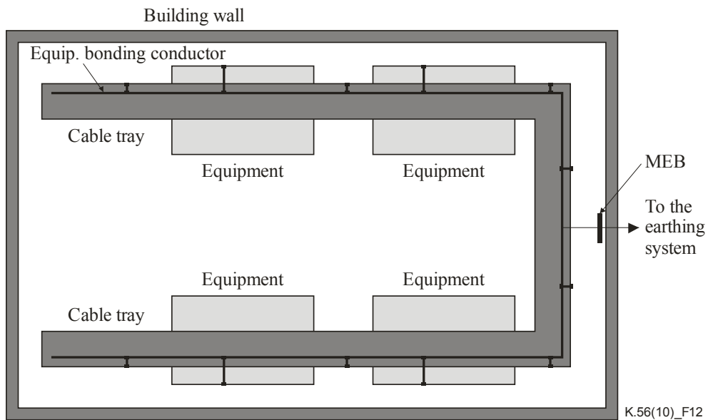
Figure 12 – Equipotential bonding conductor in the cable trays
