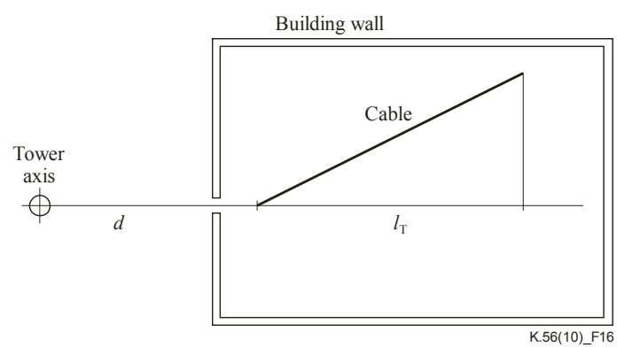
Figure 16 – Plan view representation of the distance d and length l_T
