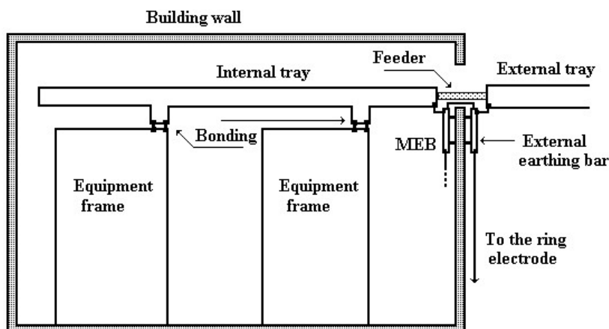
Figure 14 – Lateral view of the RBS showing the bonding between internal tray and equipment frame
