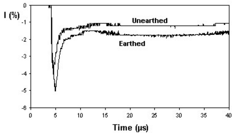
Figure I.4 – Feeder current as a function of the bonding procedure at ground level
