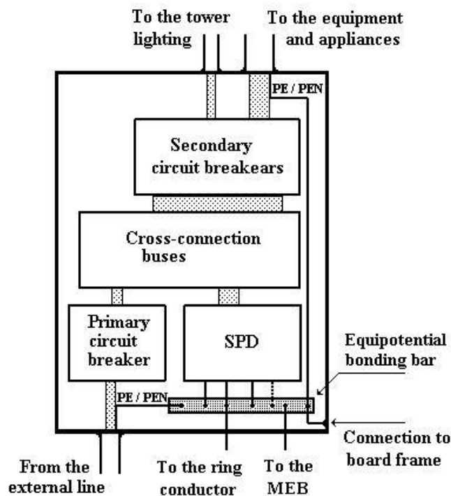
Figure 7 – Diagram of the electric board
