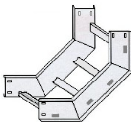
Figure 3 – Curved section used to maintain the continuity of the feeder tray
