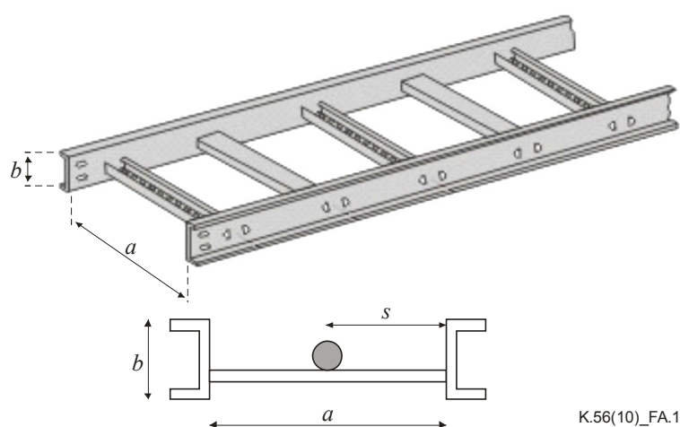
Figure A.1 – Ladder cable tray
