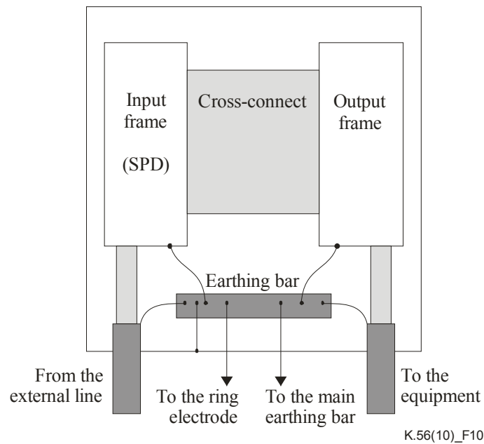
Figure 10 – Diagram of the telecommunication distribution frame
