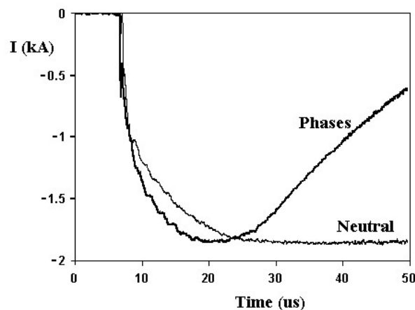
Figure I.5 – Currents in the power conductors for the fast-rising stroke current
