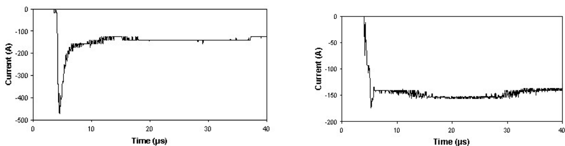
Figure I.3 – Feeder currents for fast-rising (left) and slow-rising (right) stroke currents
