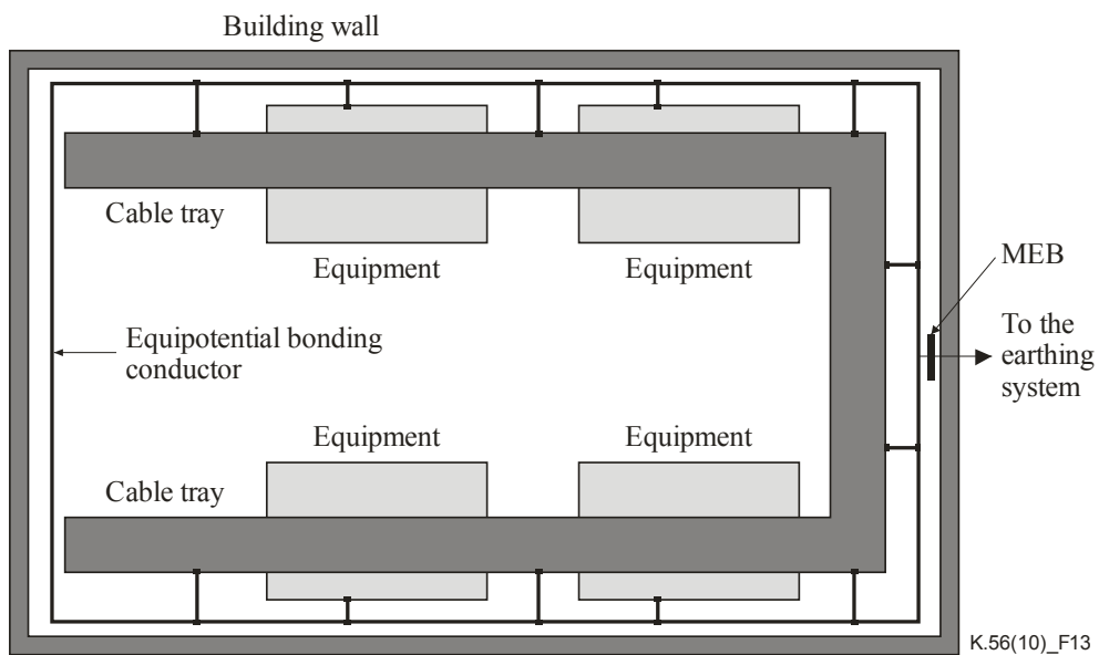
Figure 13 – Equipotential bonding conductor around the equipment room
