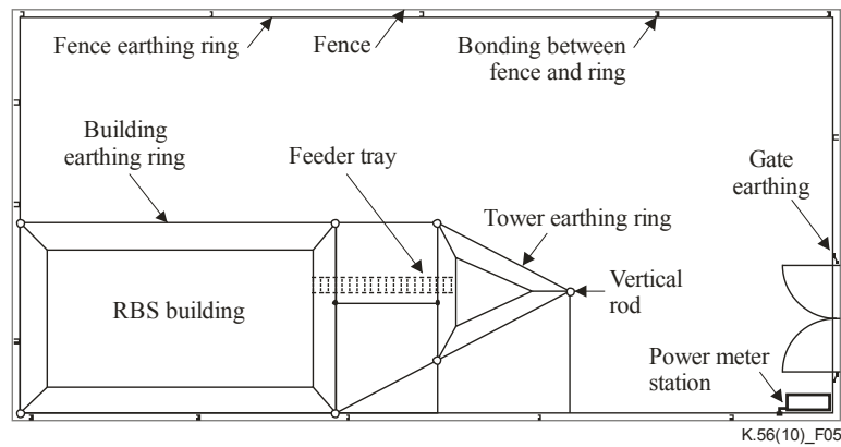
Figure 5 – Earthing system of the RBS
