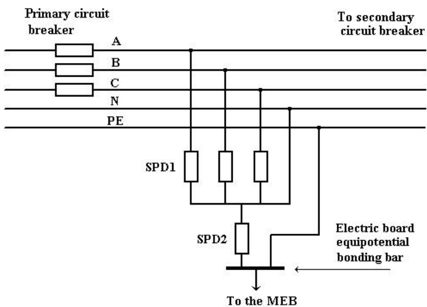
Figure 9 – Schemes for SPD installation on TN-S, TT or IT power systems
