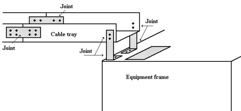
Figure 15 – Detail of the electrical continuity in trays and equipment frame
