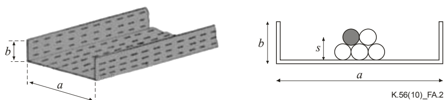
Figure A.2 – Channel cable tray
