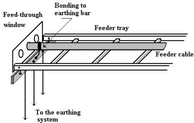
Figure 6 – Example of earthing the feeder cable at the feed-through window
