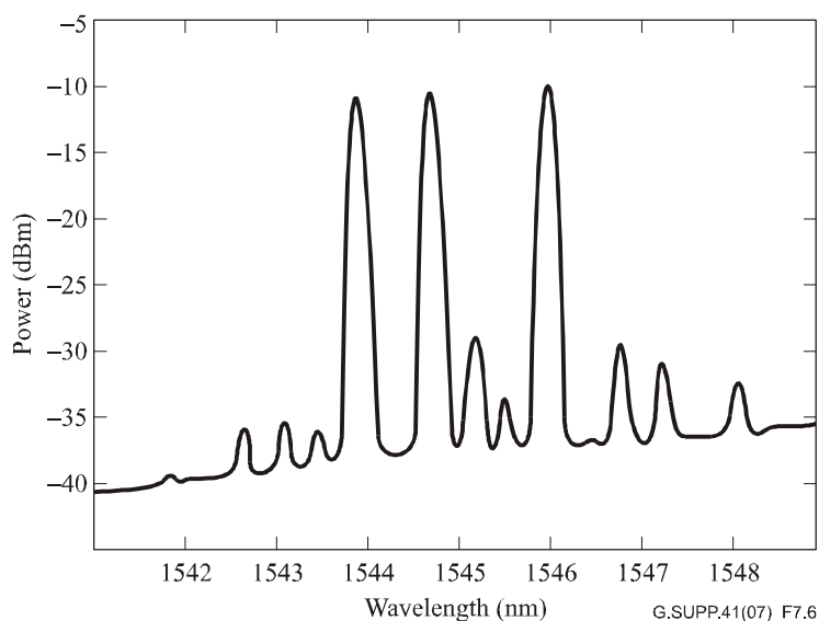
Figure 13 – Optical power spectrum measured at the output of 25 km length of dispersion shifted ( D = -0.2 ps/nm · km at the central channel) when 3 mW channels are used [b-Tkach]
