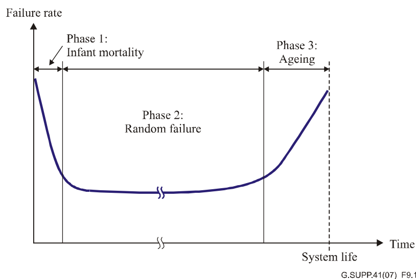
Figure 18 – Typical failure rate behaviour during the life of a system
