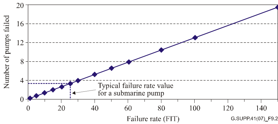
Figure 19 – Estimated number of pumps failed in 25 years for a typical transatlantic link composed of one fibre pair and 150 repeaters containing four pumps each
