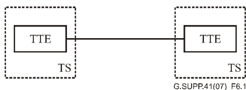
Figure 1 – Point-to-point topology
