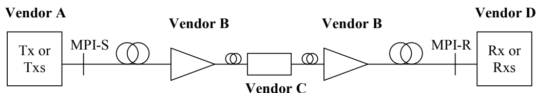
Figure 24 – Multi-span black-box full transverse compatibility
