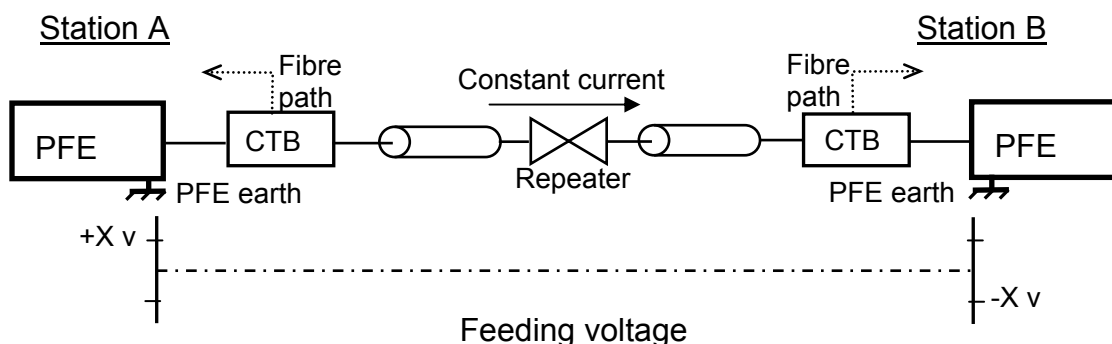
Figure 16 – Double-end feeding
