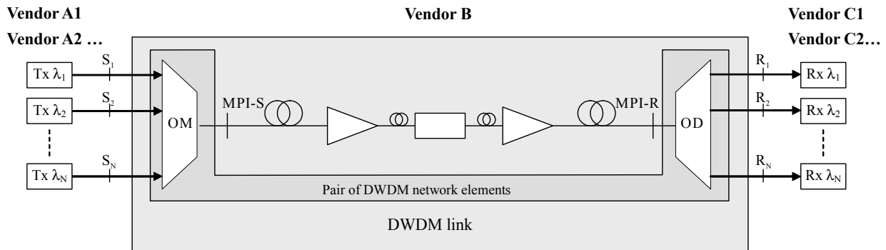
Figure 28 – Multi-span black-link transverse compatibility
