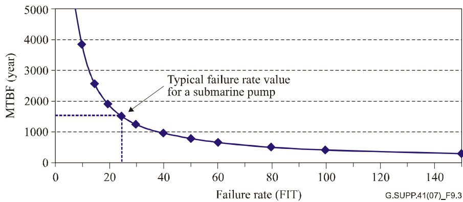
Figure 20 – MTBF for a second pump failure in the same repeater in a typical transatlantic link composed by one fibre pair and 150 repeaters with four redundant pumps each
