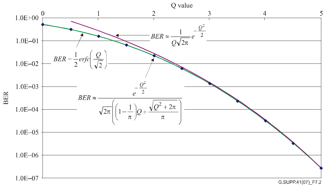
Figure 9 – Approximations relating BER and Q
