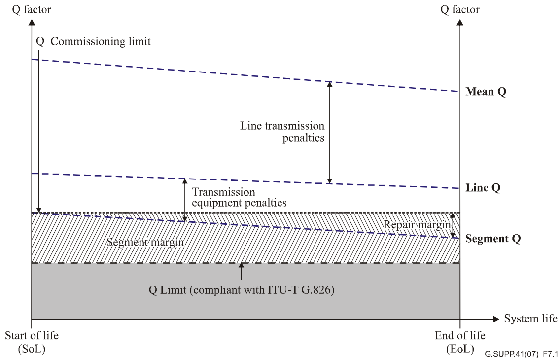
Figure 8 – Power budget structure example
