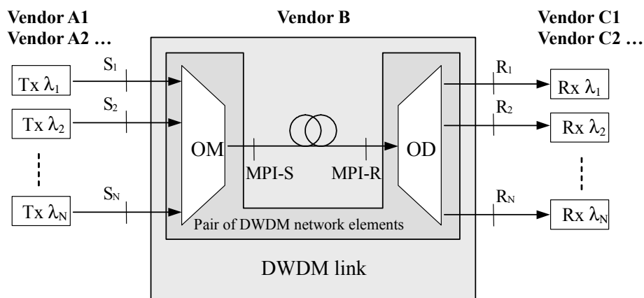
Figure 27 – Single-span black-link transverse compatibility
