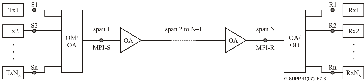
Figure 10 – Representation of optical line system interfaces (a multichannel N-span system)
