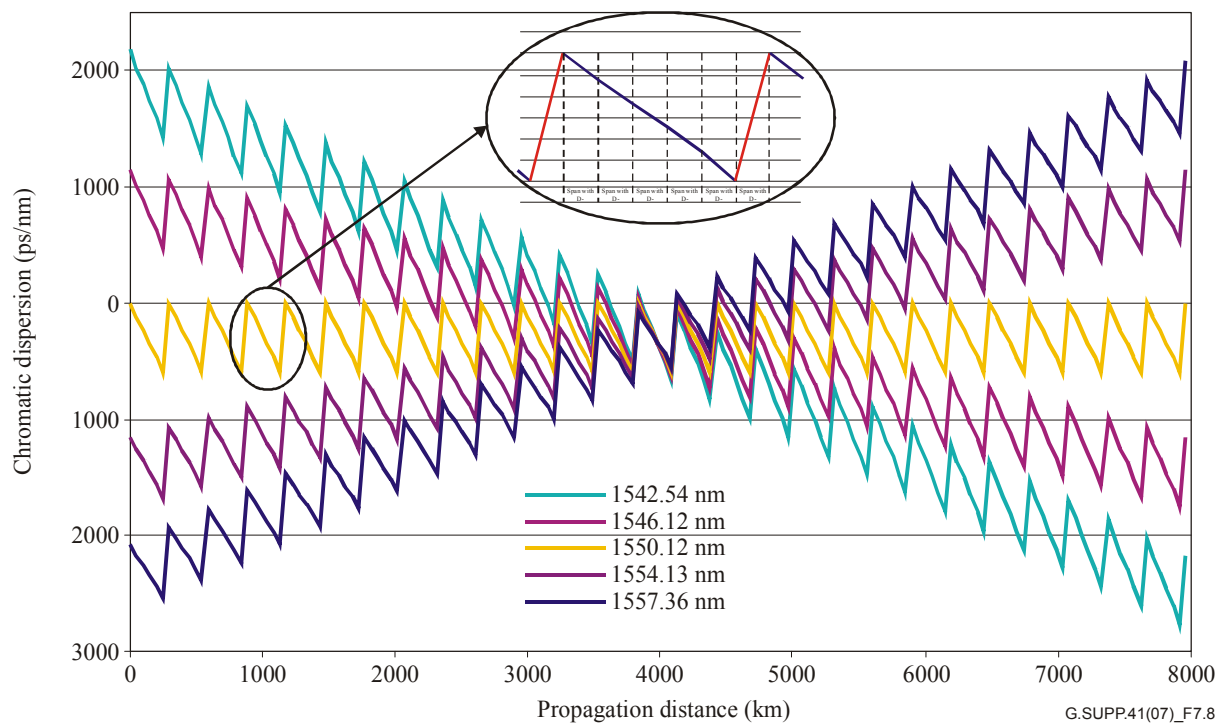
Figure 15 – Typical chromatic dispersion map for a submarine WDM system with 163 spans designed for 40 wavelengths centred around 1550.12 nm
