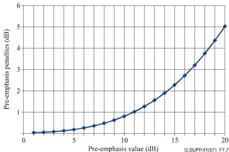
Figure 14 – An example of penalties induced by the pre-emphasis adjustment
