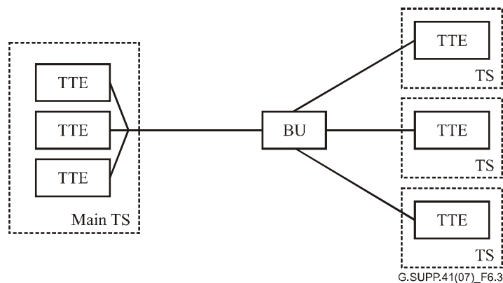
Figure 3 – Branched star topology
