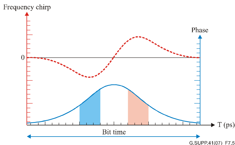
Figure 12 – Temporal variation of the phase shift and the frequency chirp induced by SPM [b-Agrawal]
