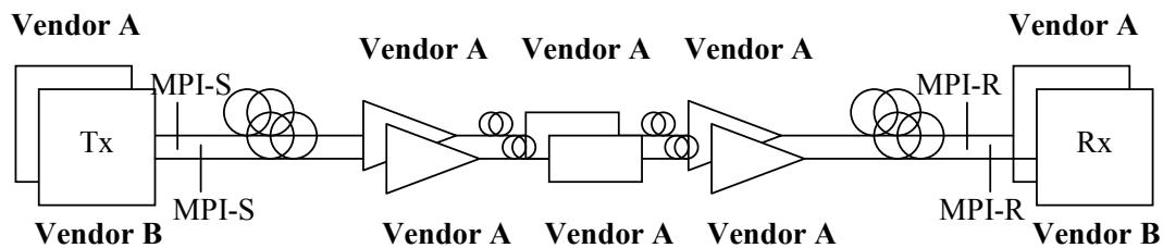
Figure 26 – Multi-span black-box multiple-link transverse compatibility
