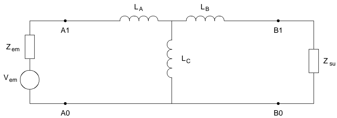
b) Shielding model for intra-CBN coupling
