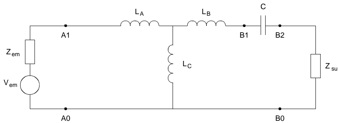
c) Shielding model for CBN-IBN coupling
