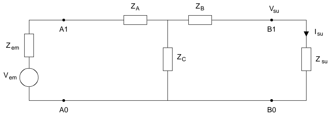
a) Fundamental shielding model
