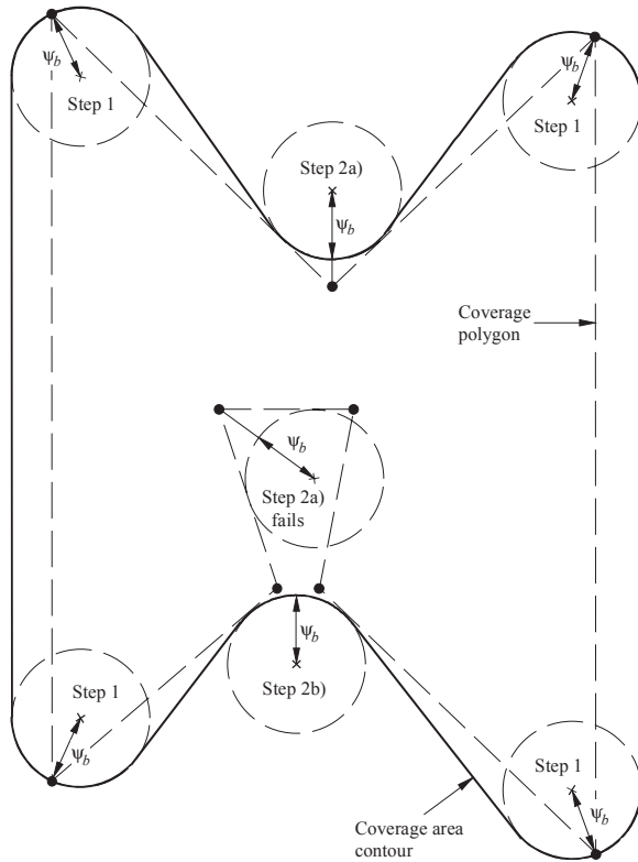
FIGURE 7 Construction of a coverage area contour
