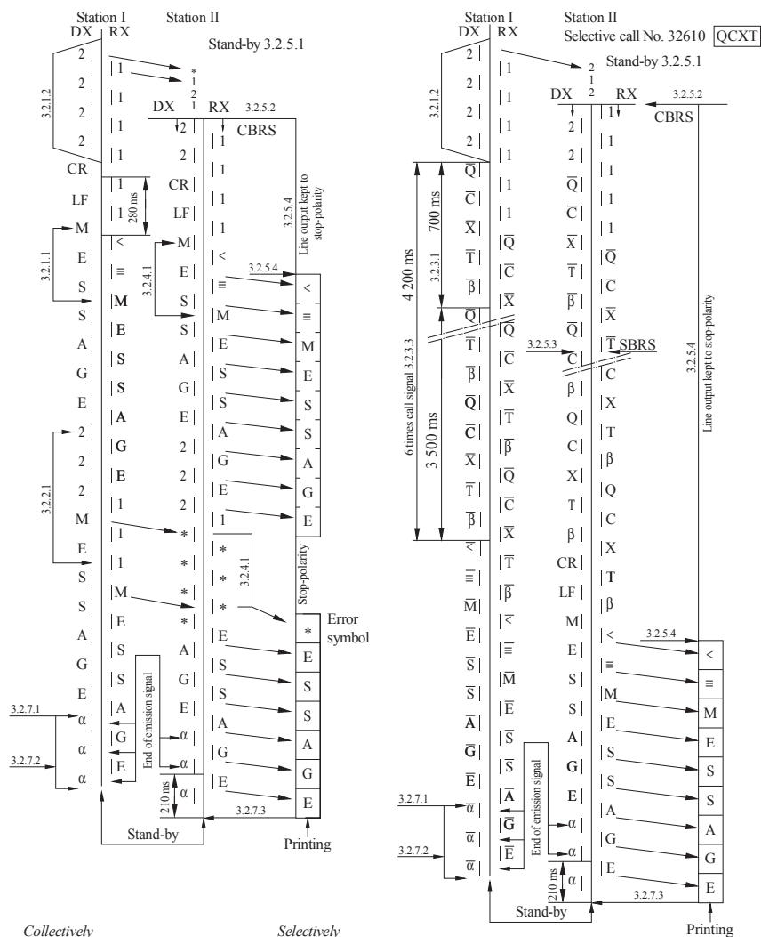
FIGURE 3 B-mode operation
