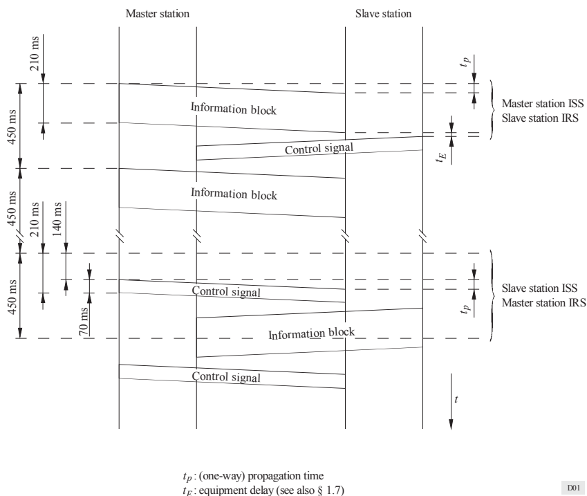
FIGURE 1 Basic timing diagram
