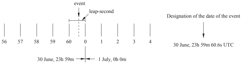
FIGURE 3 Positive leap-second
