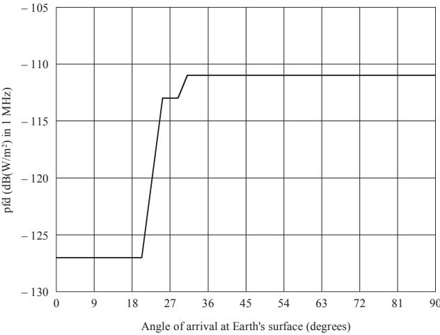
FIGURE 1 Maximum satellite pfd limits (ALS, MPR and RSMS)
