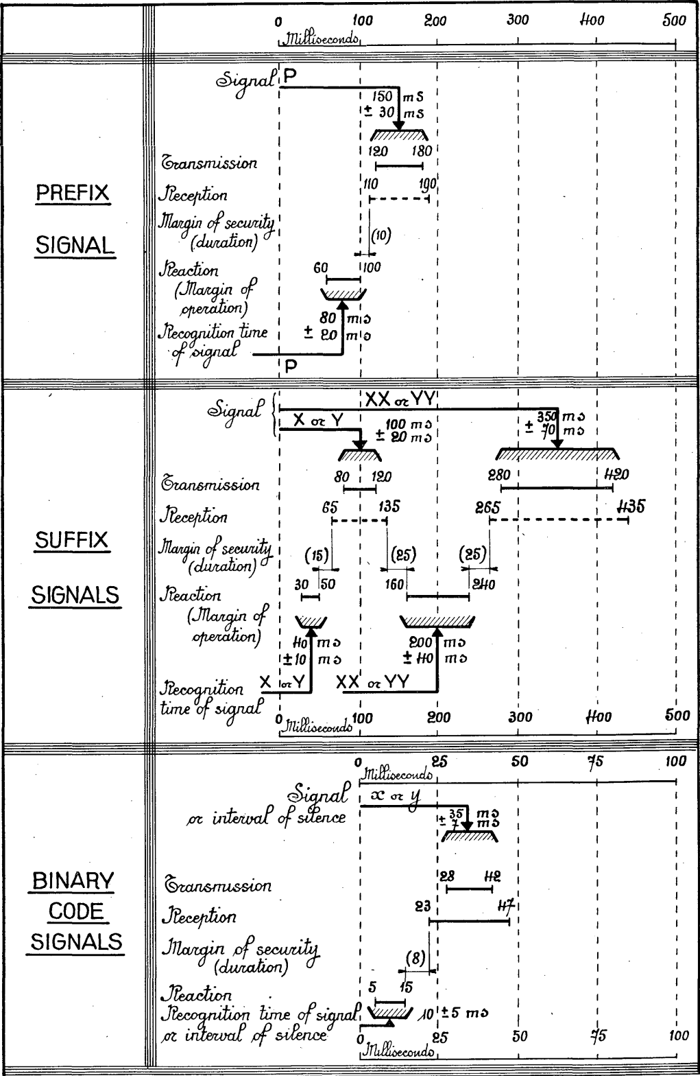
FIGURE 4 — (Binary-code signals).
