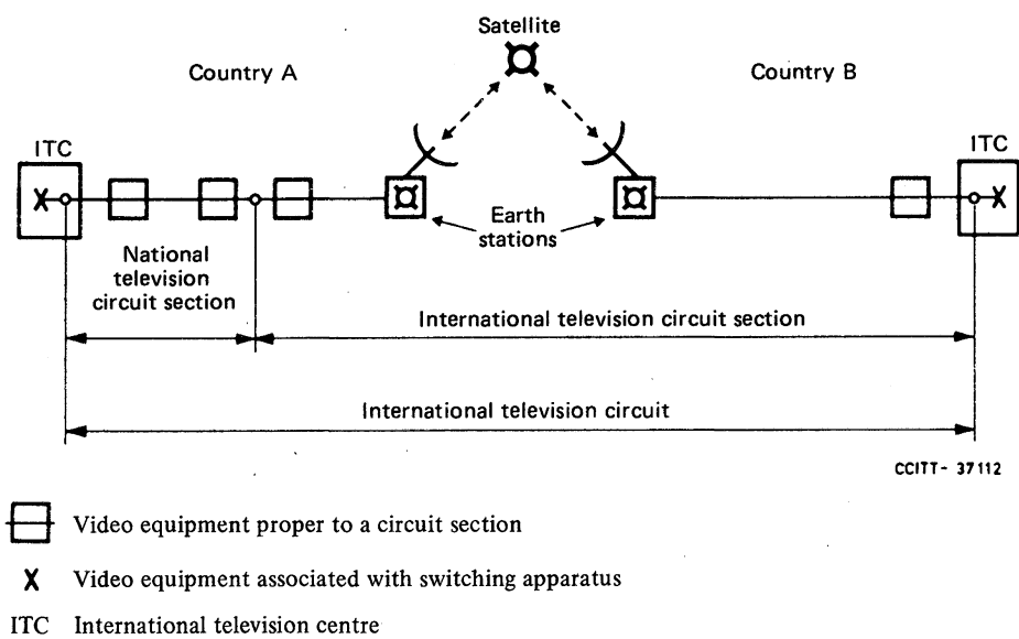
FIGURE 3/N.51 Single destination international television circuit routed via a communications satellite
