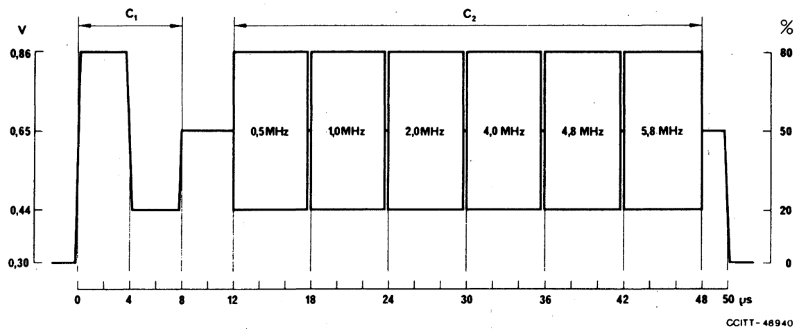
FIGURE A-5/N.73 Signal C for 625-line circuits
