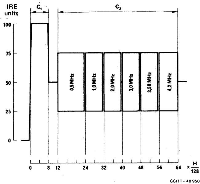
FIGURE A-6/N.73 Signal C for 525-line circuits
