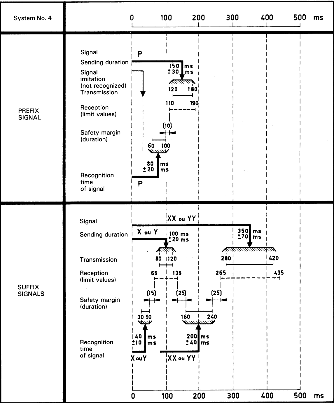
FIGURE 1/Q.121 Duration of Line Signal Elements
