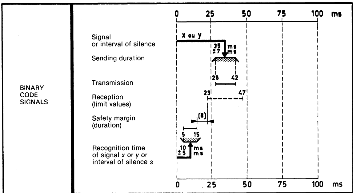
FIGURE 2/Q.121
