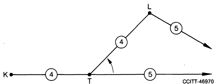
FIGURE 2/Q.180
