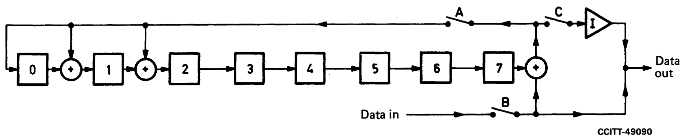
Typical shift register coder implementation
