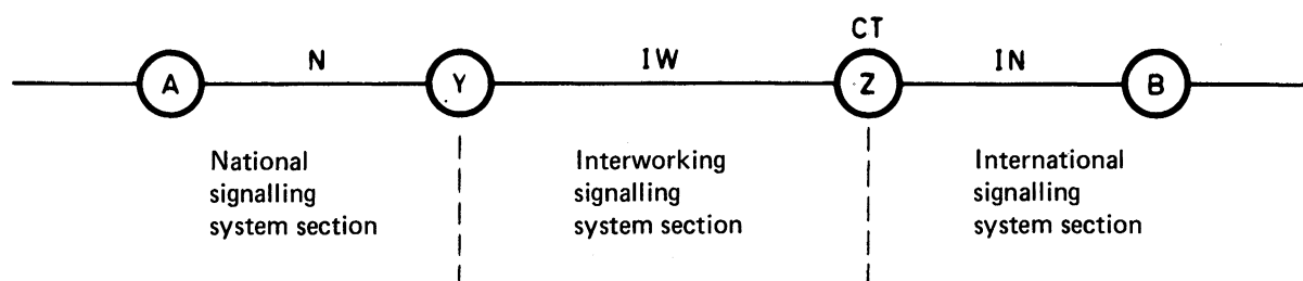
FIGURE 2/Q.300 Interworking point, example 2
