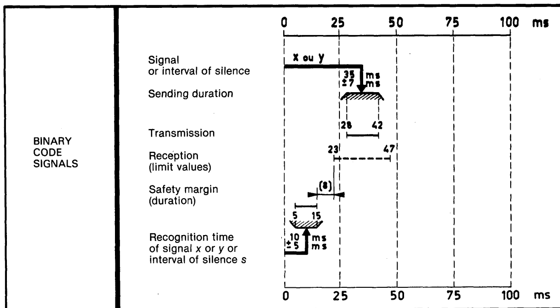
FIGURE 2/Q.121
