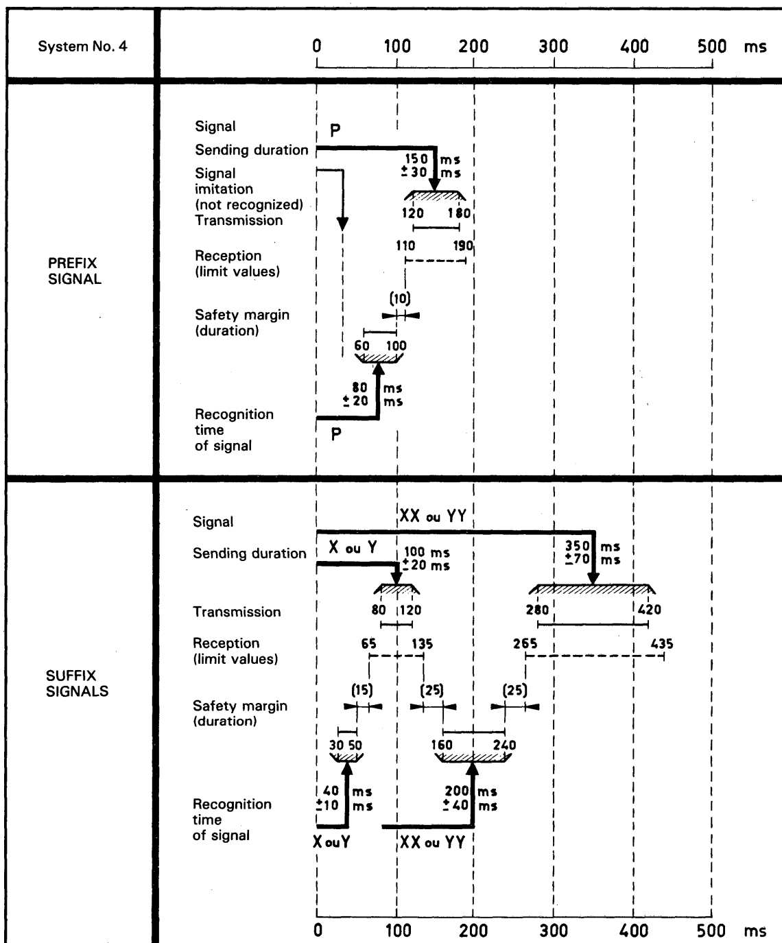
FIGURE 1/Q.121
