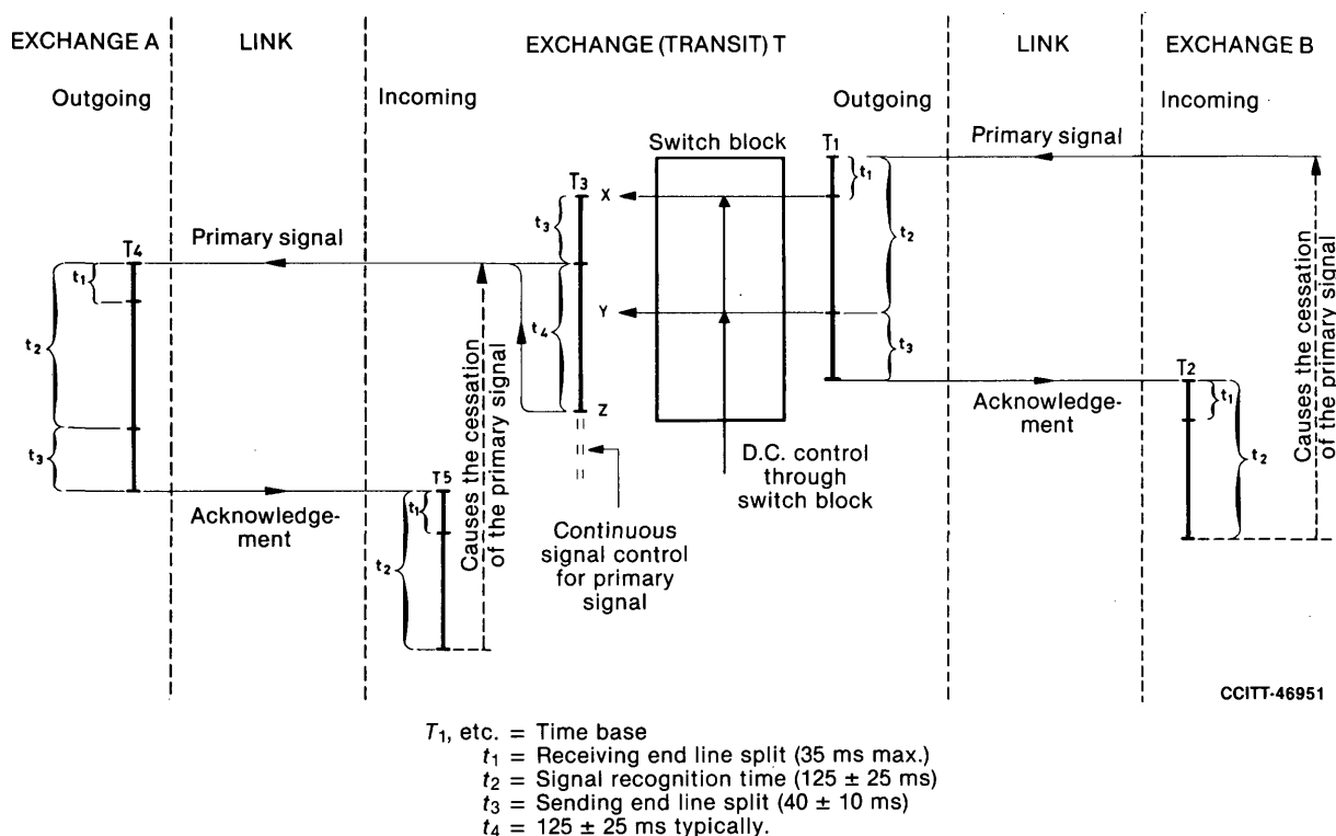
FIGURE 1/Q.141
