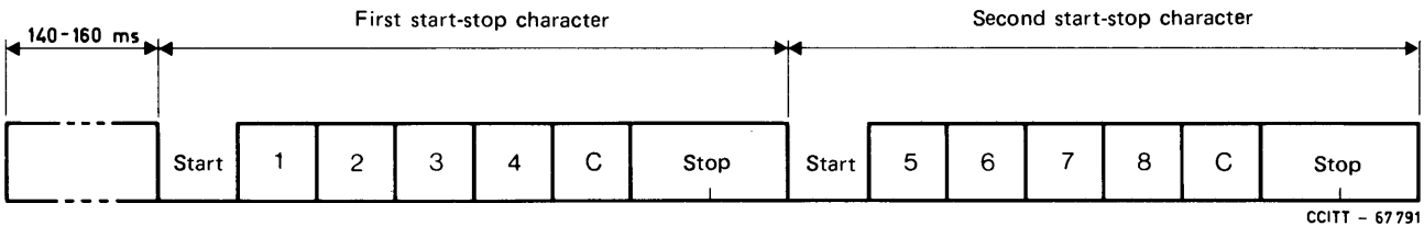
FIGURE 1/R.105 Structure for transmission of the conventional number in the virtual channel
