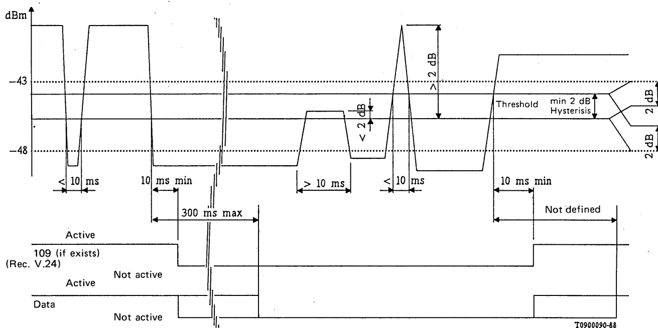
FIGURE 1/R.20 Receive signal level and reaction of the equipment
