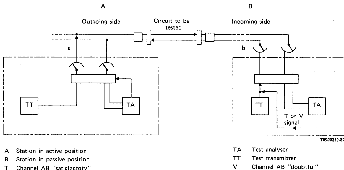
FIGURE 1/R.79 Typical equipment block diagram for automatic testing of transmission quality on telegraph circuits
