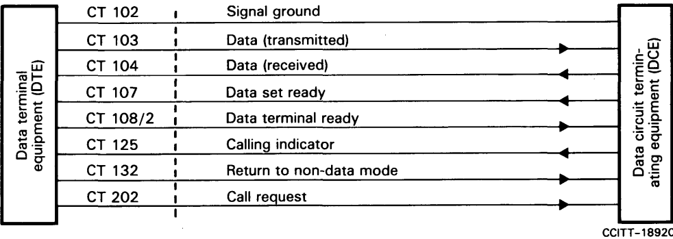
FIGURE 2/S.16 Interface for automatic calling (keyboard selection)
