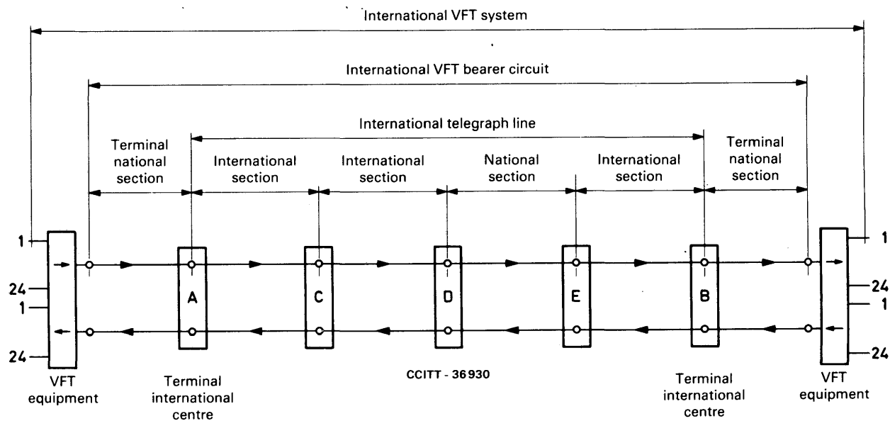
FIGURE 1/R.77 The components of an international VFT system
