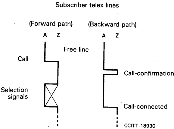
FIGURE 2/S.19 Type B call establishment
