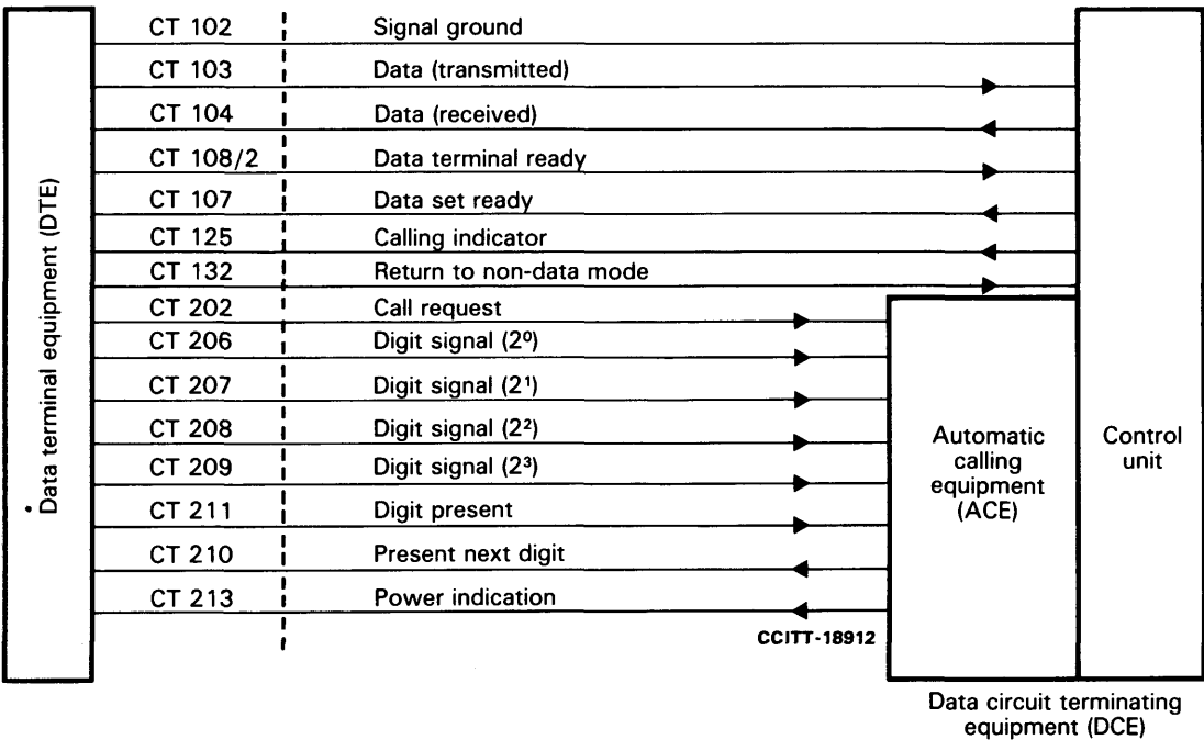
FIGURE 1/S.16 Interface for automatic calling (dial selection)
