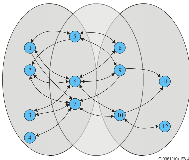
Figure 8-41 – Example 12-node network showing topology coverage ellipses and optimal paths
