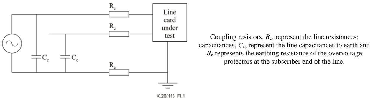
Figure I.1 – Test set-up for a line card in a telecommunication centre to simulate earth potential rise at the subscriber end
