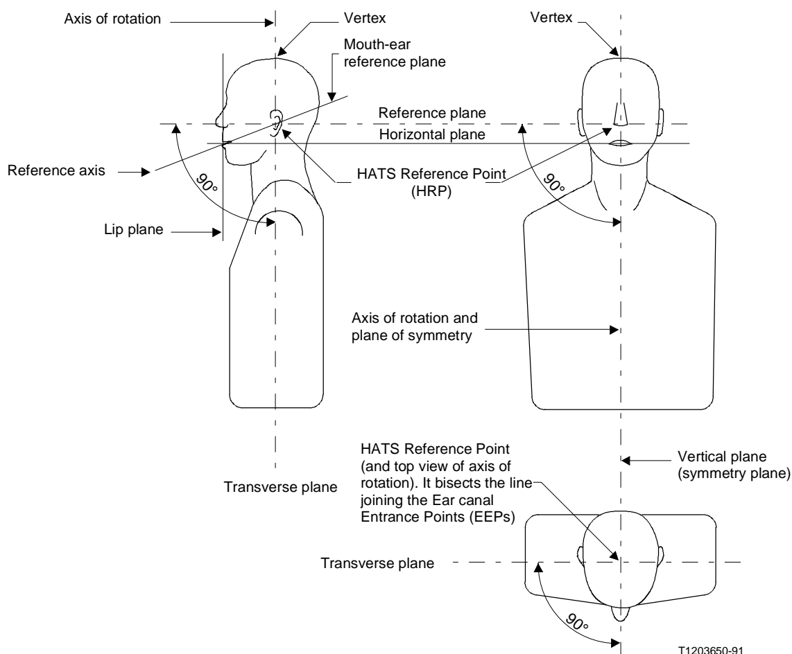
FIGURE 1/P.58 HATS geometrical references
